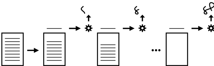
Fig. 1: Interpreted/Scripted Execution
